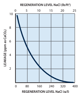
Fig. 5 HARDNESS LEAKAGE
